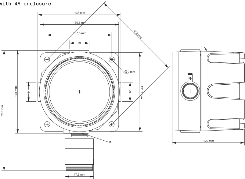
Mechanical drawings SMART S-SS with 4A enclosure
