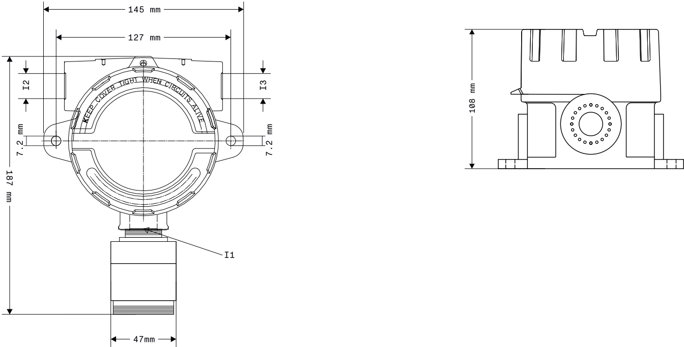
Mechanical drawings SMART S-SS with 4A enclosure
