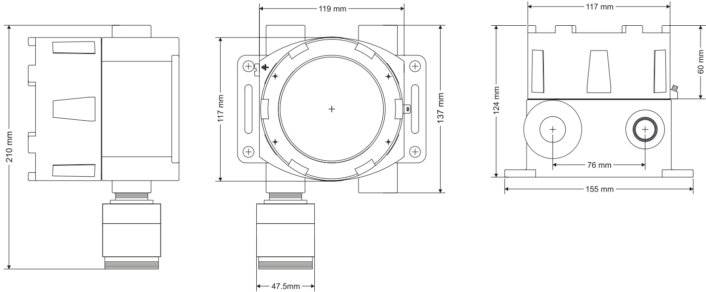
Mechanical drawings SMART S-SS with 2S enclosure
